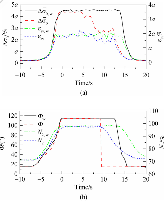
图 4 有、无尾喷流吸入时发动机进口总压畸变指数对比 Fig. 4 Comparison of total pressure distortion indicators between conditions with and without exhaust gas ingestion
